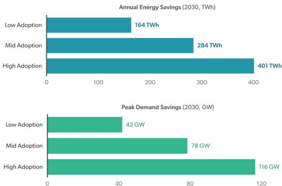
Figure 3. Potential Value to the U.S. Power System of Peak Demand and Energy Savings from Different GEB Adoption Levels (Source: DOE GEB Roadmap 2021)
